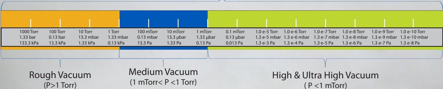
Vacuum Measurement Range
